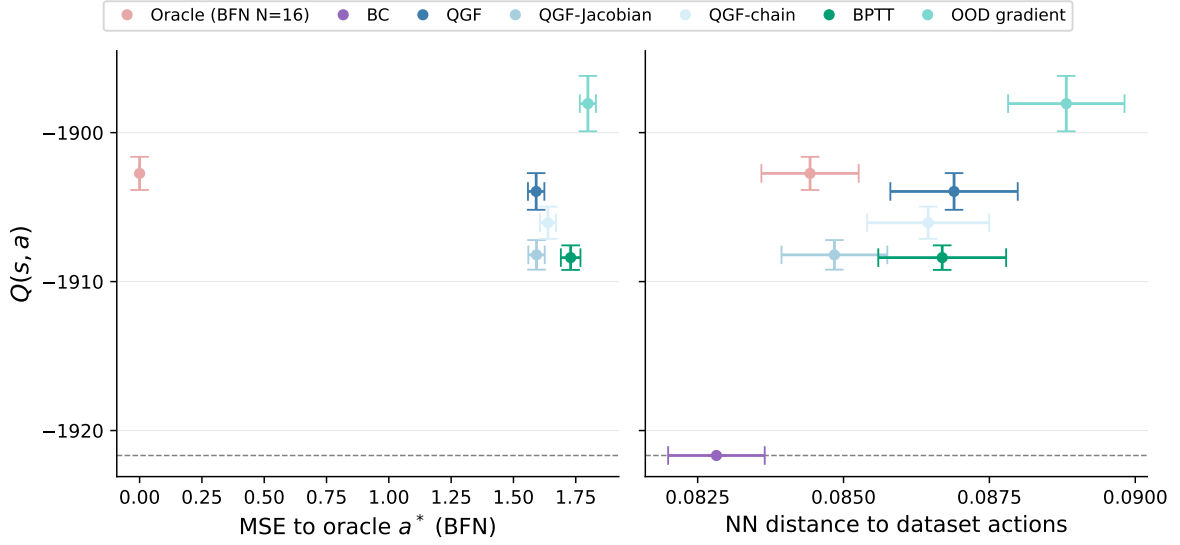
Figure 17: The OOD gradient leads to a denoised action with higher Q value than all other methods by exploiting the critic on OOD actions. (left): the OOD gradient leads to actions that are farthest away from the BFN oracle actions. (right): the OOD gradient leads to actions that has the largest nearest-neighbor (NN) distance to dataset actions. Aggregated over 20 tasks, 256 observations, 4 seeds.
