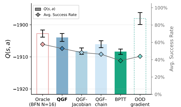
Figure 4: Q -values of the denoised action with different gradient guidance, which roughly correlate with performance. Averaged over 20 OGBench environments. QGF is the best gradient-based optimizer, getting close to the performance of the best-of-n oracle.
