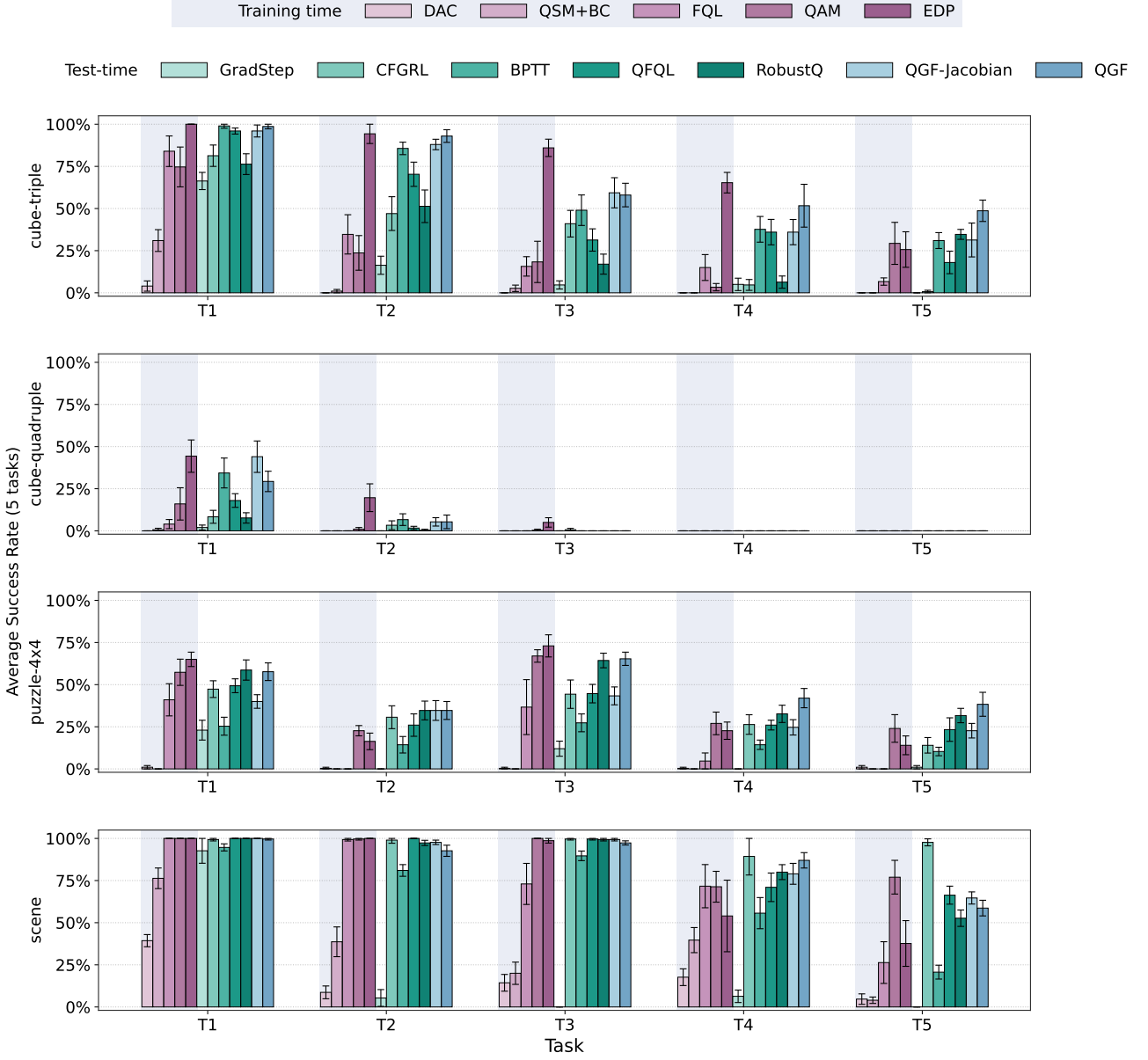
Figure 11: Offline RL performance at 500k training steps per environment (10 seeds each).
