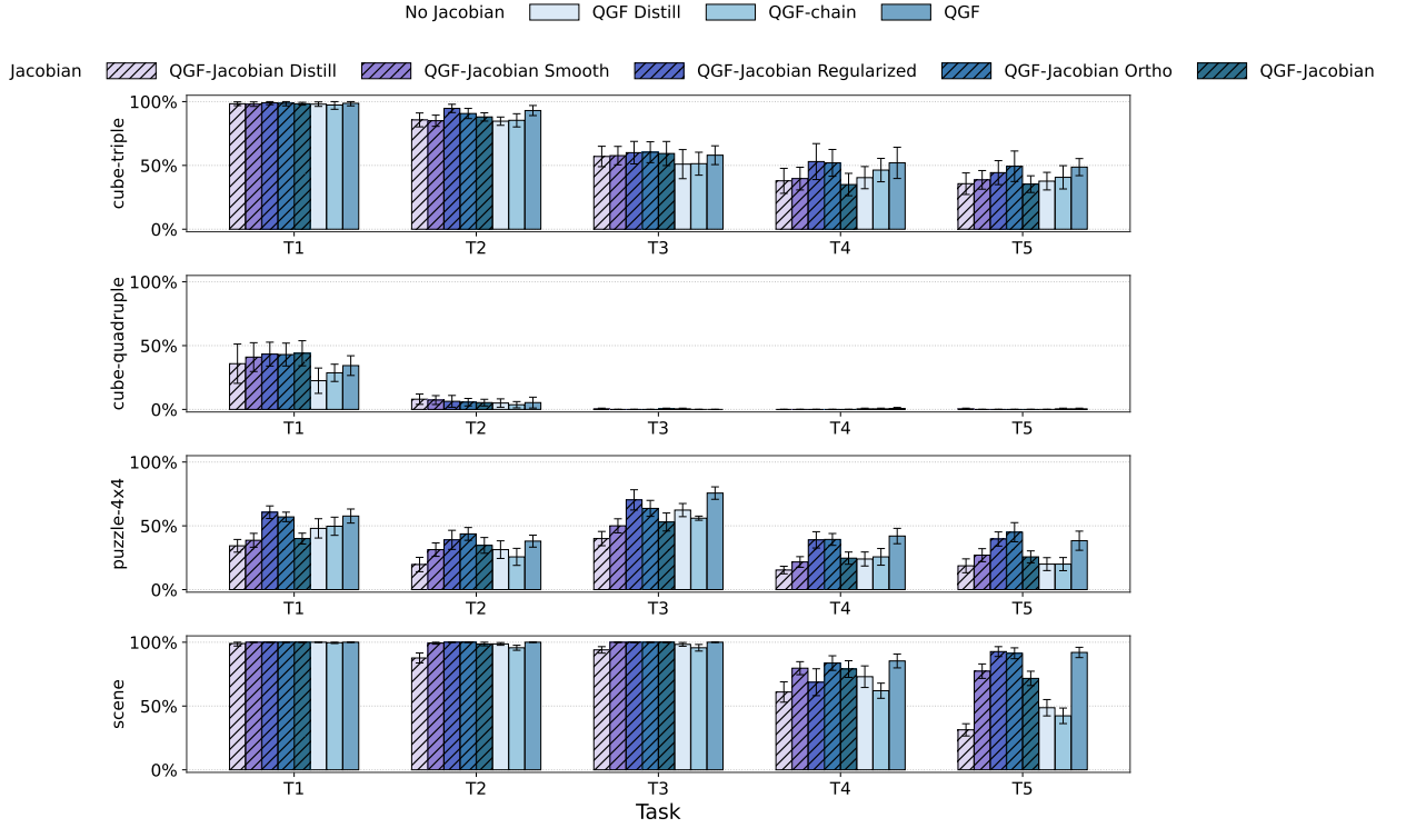
Figure 16: Full results for Fig. 15: Offline RL performance at 500k training steps (20 tasks, 10 seeds).
